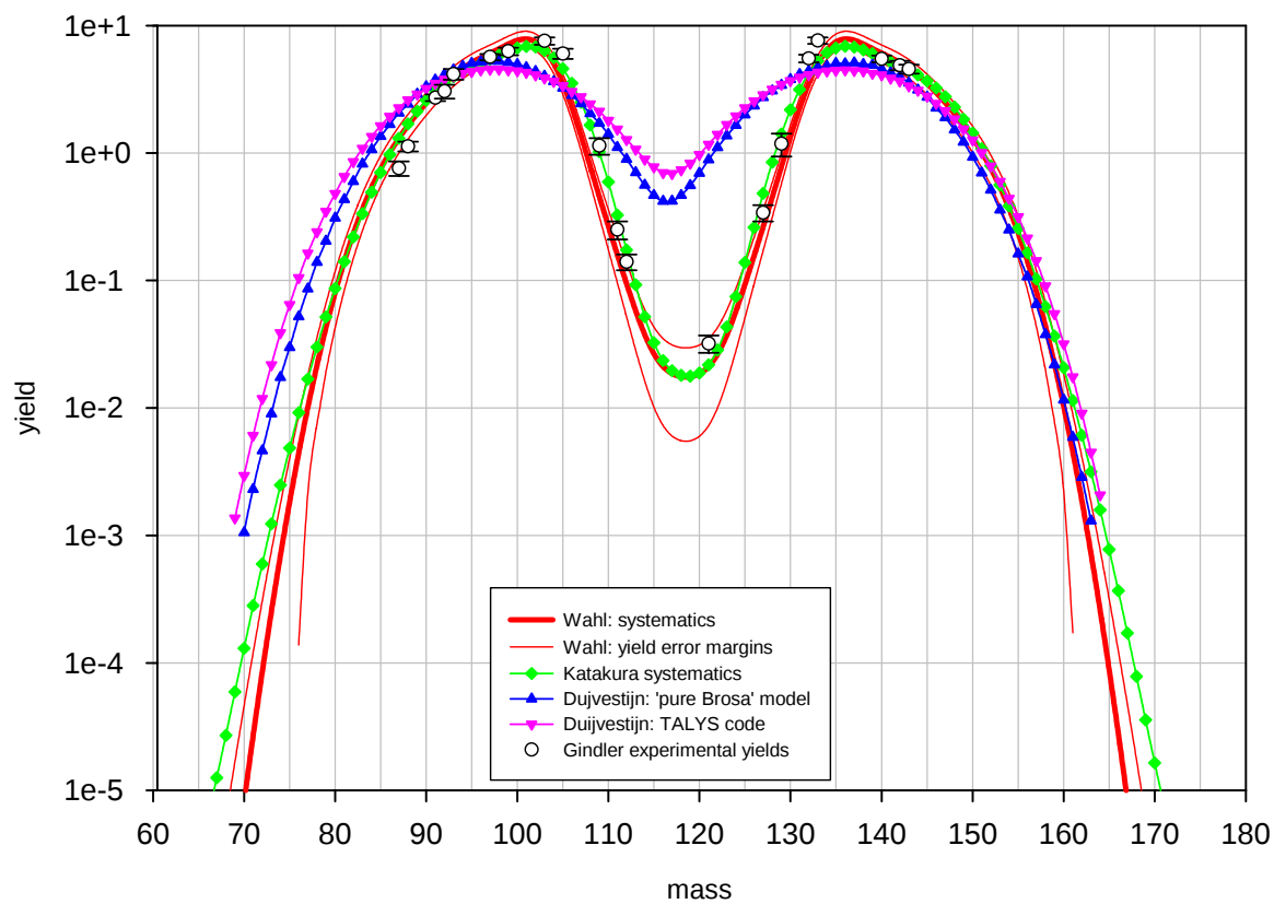
Benchmark A: ^{239}\text{Pu} at 0.17 MeV, post neutron emission yields
